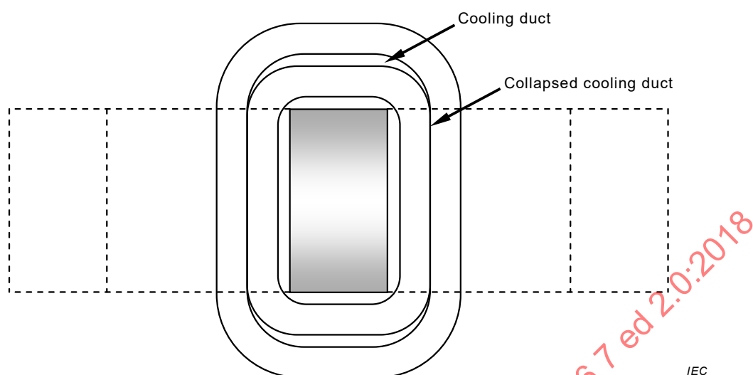
Figure 11 – Top view section of a rectangular winding with “collapsed cooling duct arrangement” under the yokes
