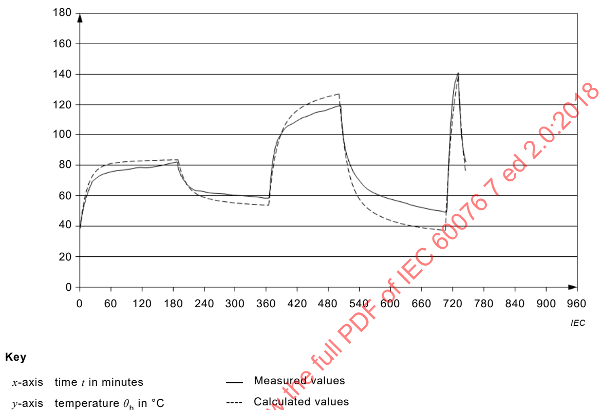
Figure H.1 – Hot-spot temperature response to step changes in the load current
