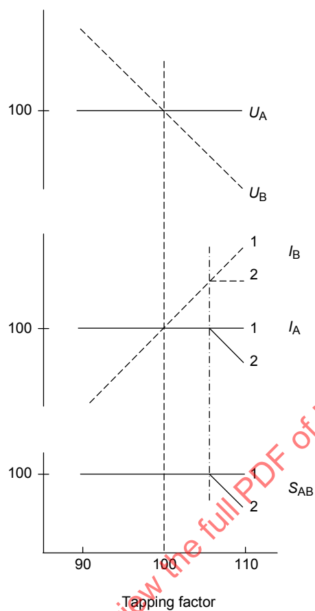
Figure 1b – Variable flux voltage variation (VFVV)
