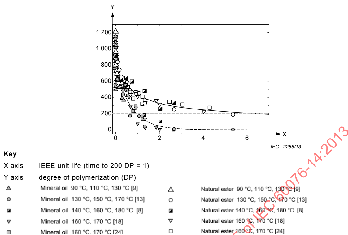
Figure C.4 – Composite DP ageing results of TUP in mineral oil and natural ester liquid
