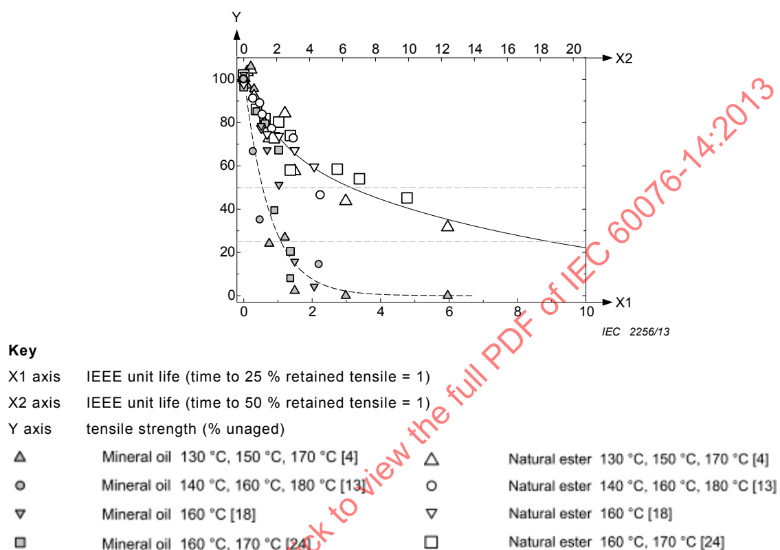
Figure C.2 – Composite tensile strength ageing results of TUP in mineral oil and natural ester liquid
