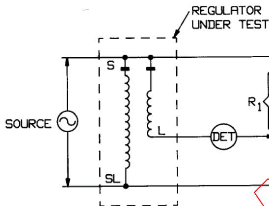
Figure 11—Basic circuit of ratio bridge
