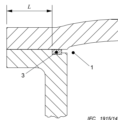
Figure 15 – Illustration of the requirements concerning gaskets – Example 6
