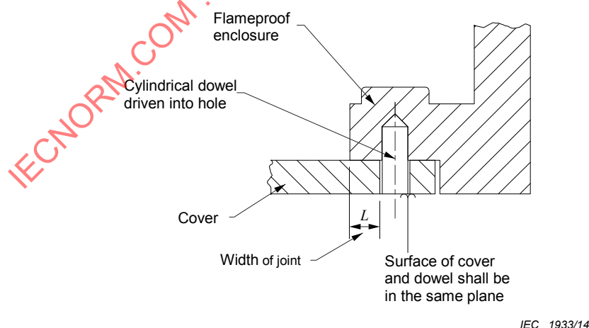
Figure 1 – Example of construction for indirect checking of a flanged Group I flameproof joint
