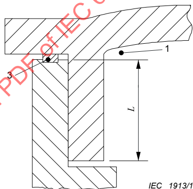
Figure 13 – Illustration of the requirements concerning gaskets – Example 4
