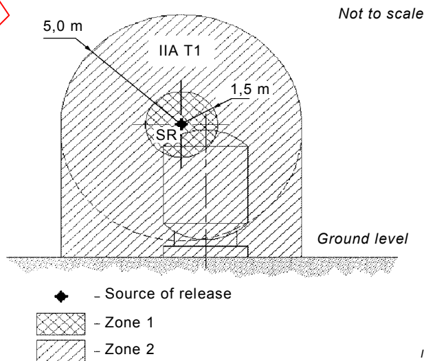
Figure E.8 – Zones classification (Example No. 3)
