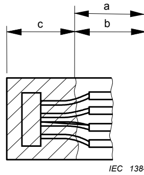
Figure 4a – Partially coated board
