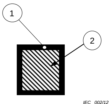
Figure D.3a – Moulding over un-mounted components
