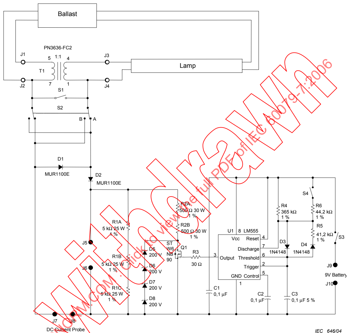
Figure H.1 – Asymmetric pulse test circuit
