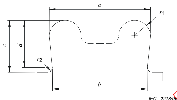
Figure 2 – Stud
