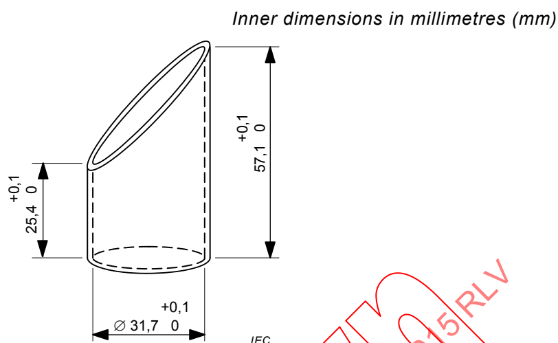
Figure 1 – Ingestion gauge
