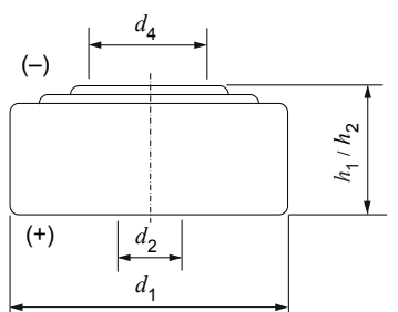
Figure 15 – Dessins des dimensions: SR62, SR63, SR65, SR64, SR60, SR67, SR66, SR58, SR68, SR59, SR69, SR41, SR57, SR55, SR48, SR54, SR42, SR43, SR44
