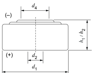
Figure 15 – Dimensional drawing: SR62, SR63, SR65, SR64, SR60, SR67, SR66, SR58, SR68, SR59, SR69, SR41, SR57, SR55, SR48, SR54, SR42, SR43, SR44
