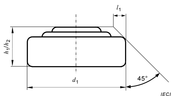
Figure 2 – Shape of negative terminal
