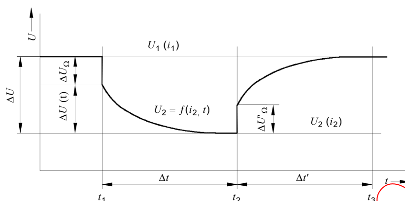
Figure 4 – Schematic voltage transient
