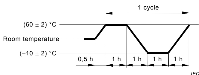
Figure 9 – Test by temperature cycles
