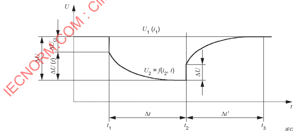
Figure 4 – Schematic voltage transient
