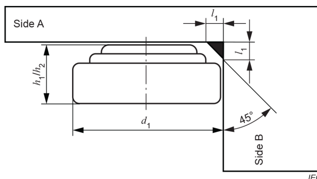
Figure 3 – Shape requirement
