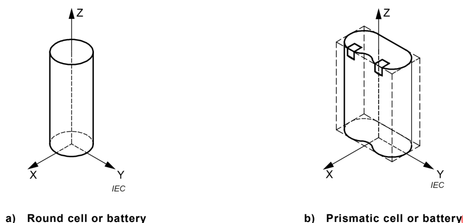
Figure 4 – Axes for free fall
