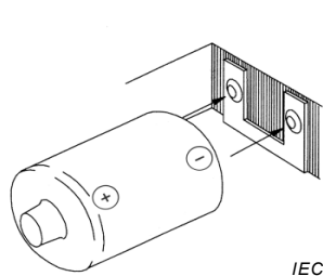
Figure B.4a – Correct insertion of the battery
