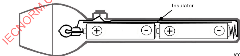
Figure B.8 – Typical example of insulation to prevent short circuit
