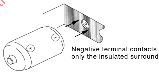
Figure B.3b – Incorrect insertion of the battery
