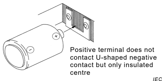
Figure B.4b – Incorrect insertion of the battery
