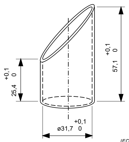
Figure 7 – Ingestion gauge (Inner dimensions)
