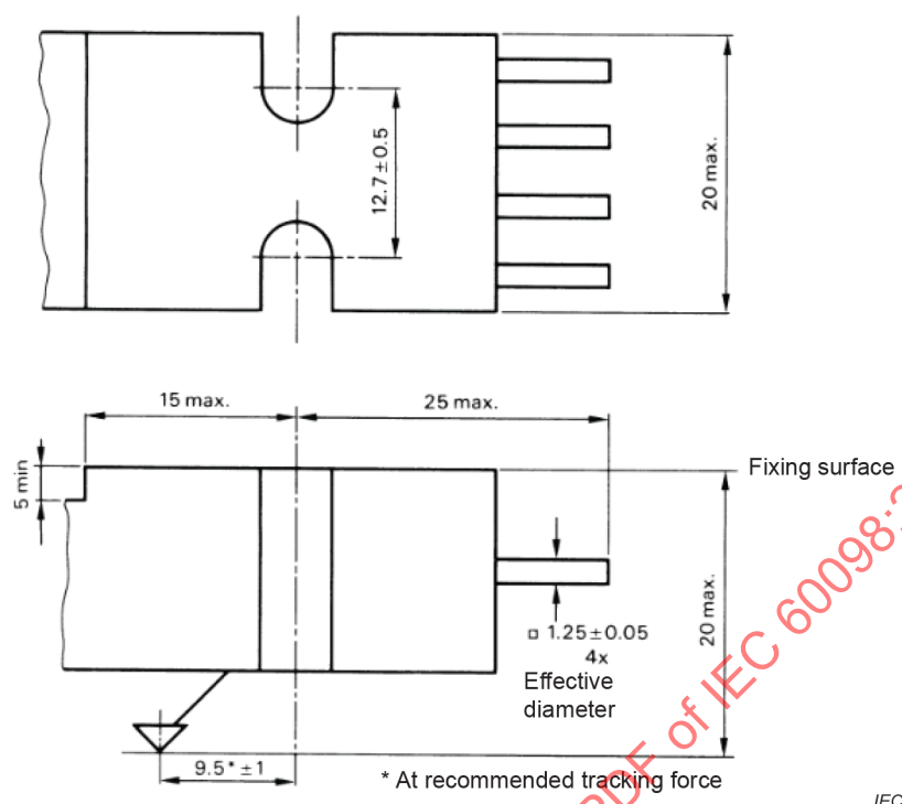
Figure 5 – Pickup cartridge
