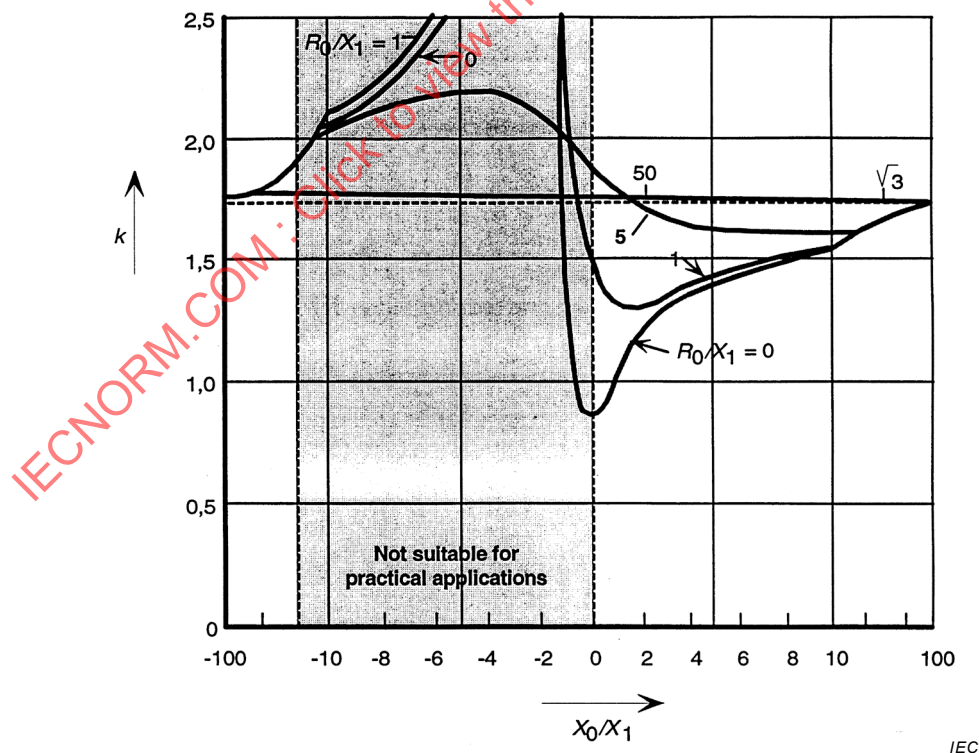
Figure A.1 – Earth fault factor k on a base of X_0/X_1 , for R_1/X_1 = R_1 = 0
