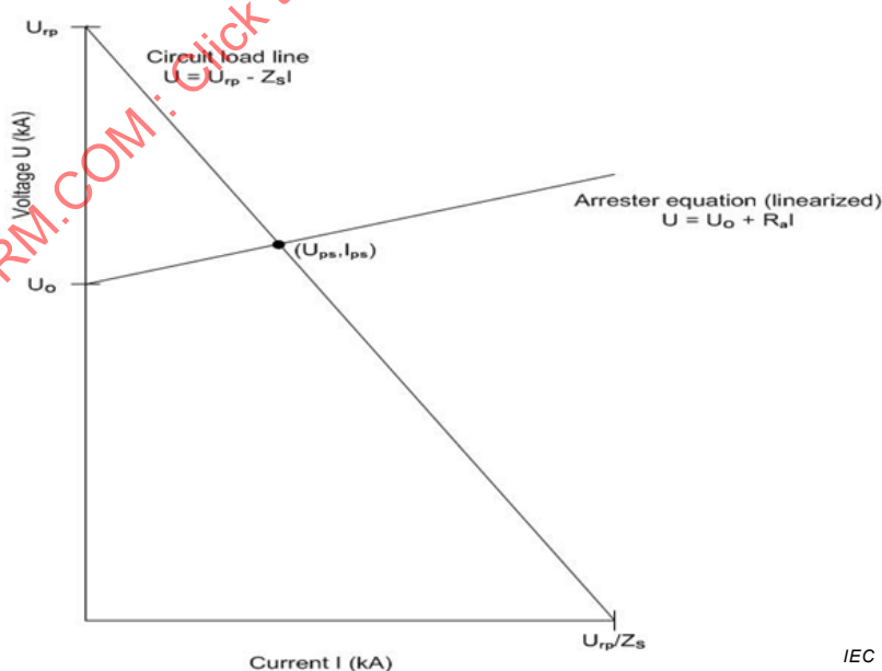
Figure I.3 – Graphical illustration of linearized line switching condition and arrester characteristic
