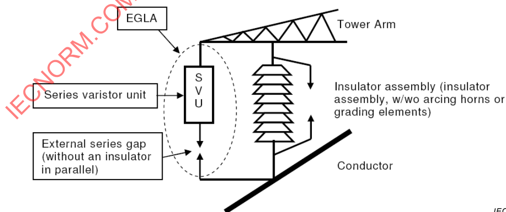
Figure 4 – Components of an EGLA acc. to IEC 60099-8
