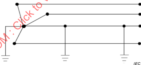
Figure 23d – Four-wire multi-earthed -wye systems. Earth Fault Factor 1,25
