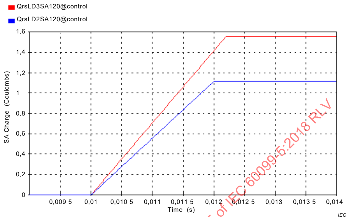
Figure I.7 – Arrester Class 2 & 3 cumulative charges calculated by EMTP simulation: Q_{rs2} and Q_{rs3} (C)
