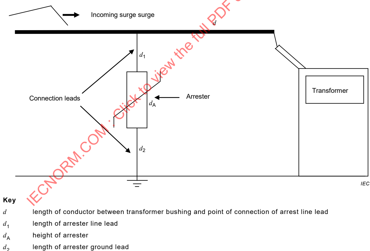
Figure C.1 – Schematic sketch of a typical arrester installation
