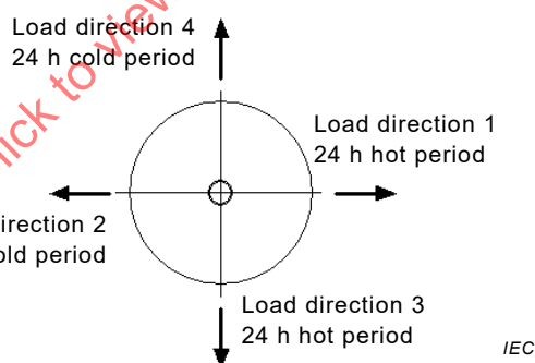
Figure 8 – Example of the test arrangement for the thermo-mechanical test and direction of the cantilever load
