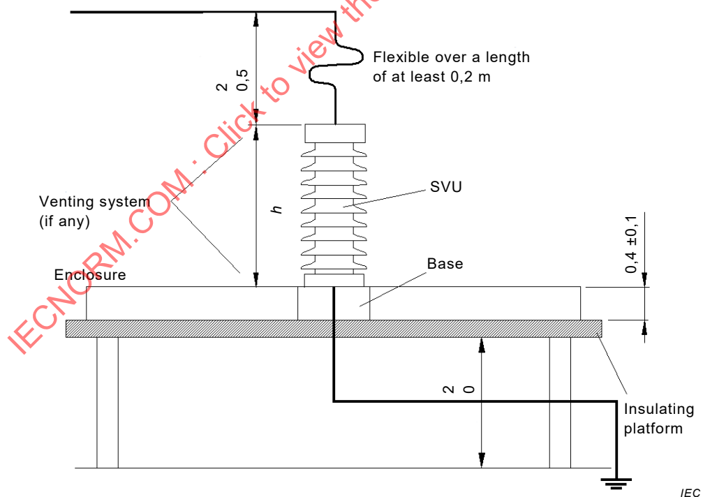
Figure 5b – Circuit layout for polymer-housed SVUs (all leads and venting systems in the same plane)
