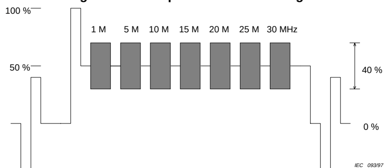
Figure 8 – Composite sine-wave signal
