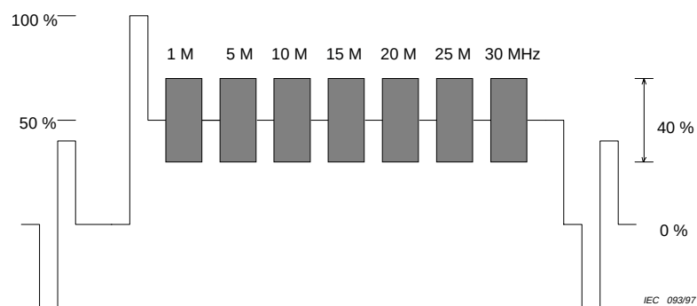
Figure 9 – Signal multisalves
