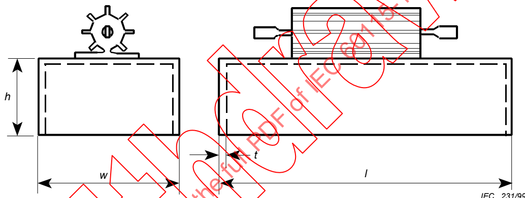
Figure 7 – Reference heat sink
