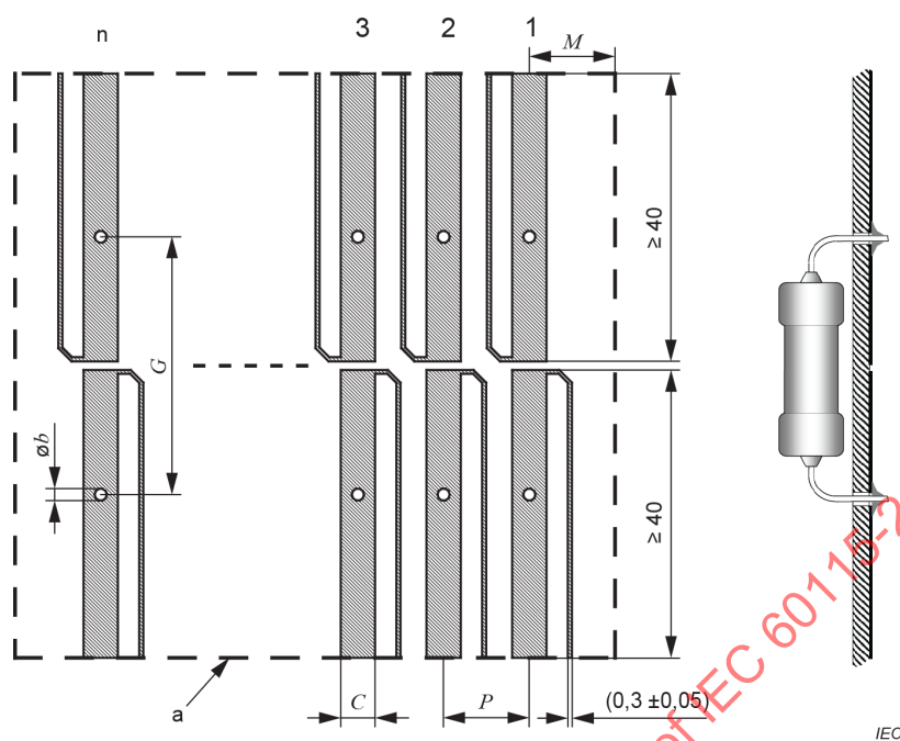
a) Basic layout with Kelvin (4 point) connections
