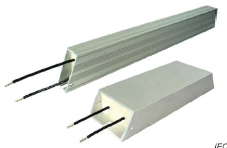
Figure 5 – Illustrations of typical metal housed power resistors
