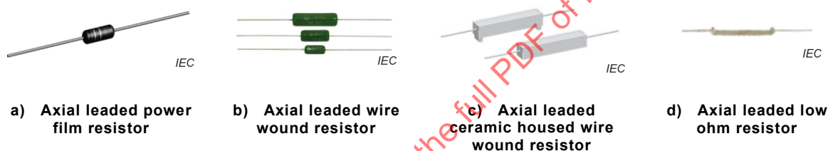
Figure 1 – Illustrations of typical axial leaded power resistors
