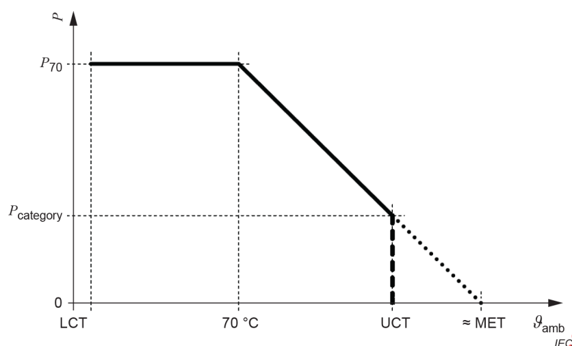
Figure 14 – Typical derating curve for MET > UCT
