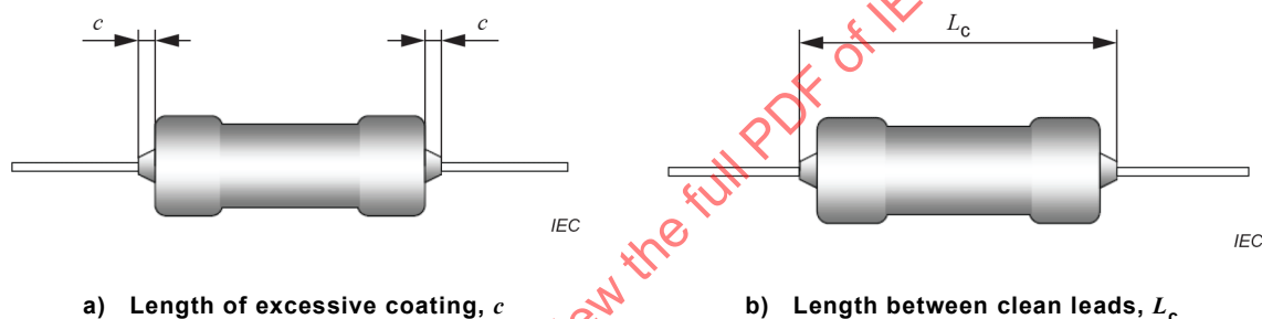
Figure 7 – Alternative methods for specification of the length of excessive protective coating or welding beads on axial leaded resistors
