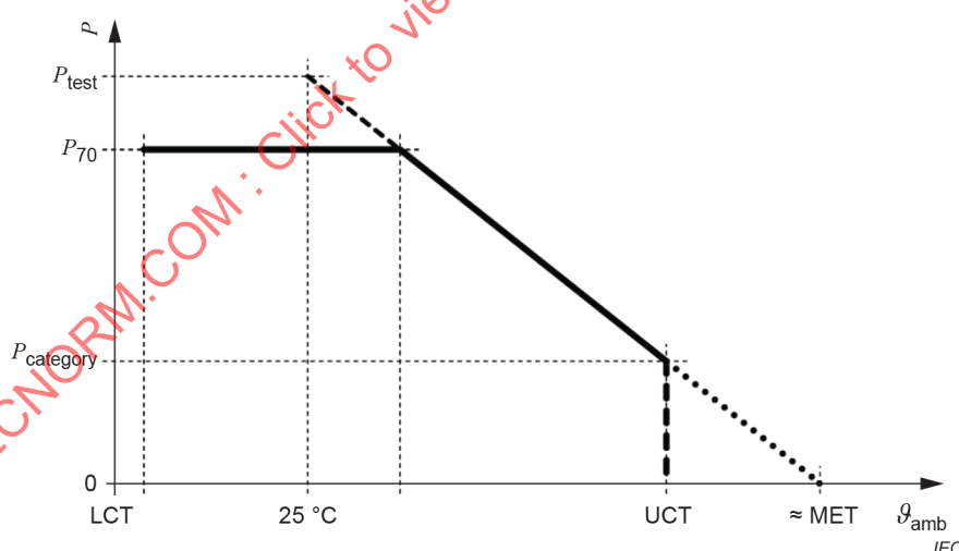
Figure 15 – Typical derating curve for power wire-wound resistors
