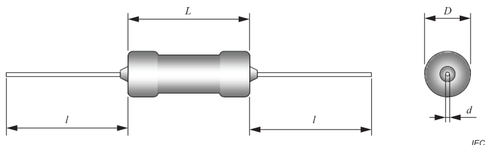
Figure 6 – Shape and dimensions of cylindrical axial leaded resistors
