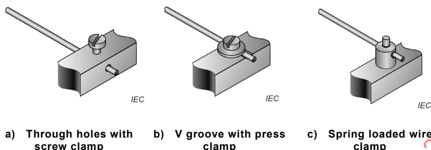
Figure 18 – Examples of specimen lead fixation devices
