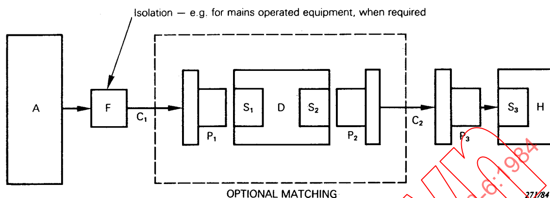
FIG. A1. — Example of a schematic circuit arrangement for connection between hearing aid and external signal source.
