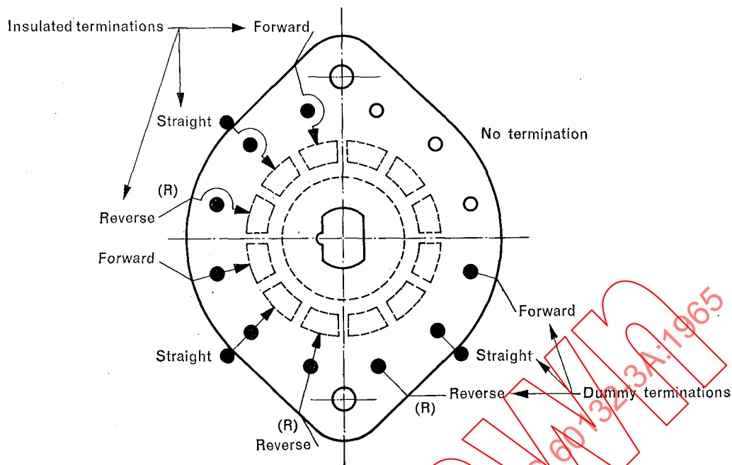
FIG. 3. — Indication of stator terminations.
