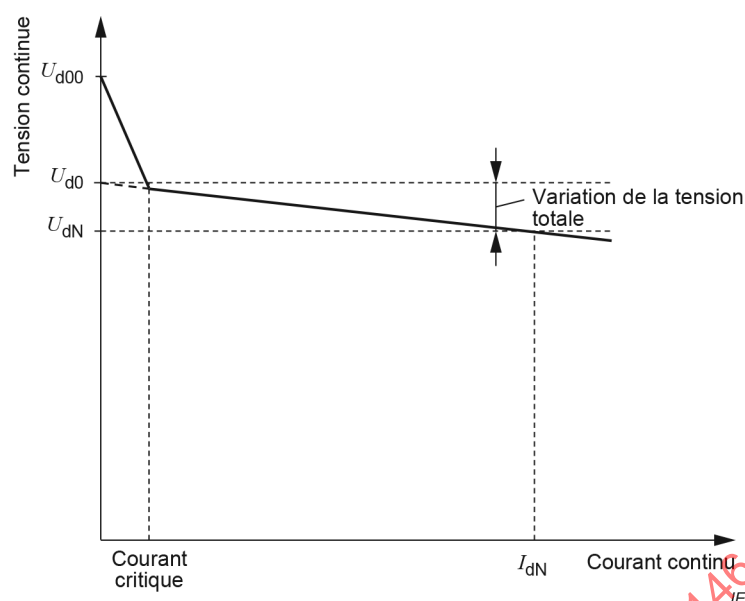
Figure 3 – Variation de tension
