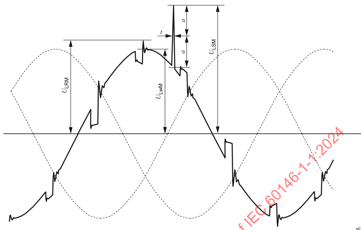
Figure 4 – AC voltage waveform
