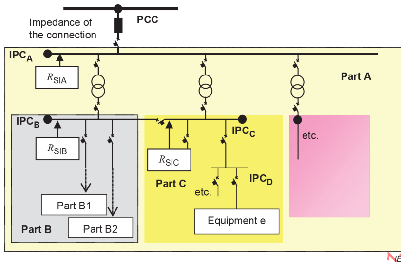
Figure B.1 – PCC, IPC, installation current ratio and R_{Sl}
