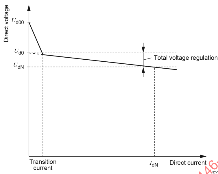
Figure 3 – Voltage regulation
