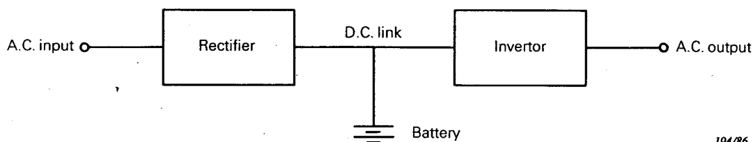
FIG. 1. — Single UPS with a common rectifier for inverter and battery.
