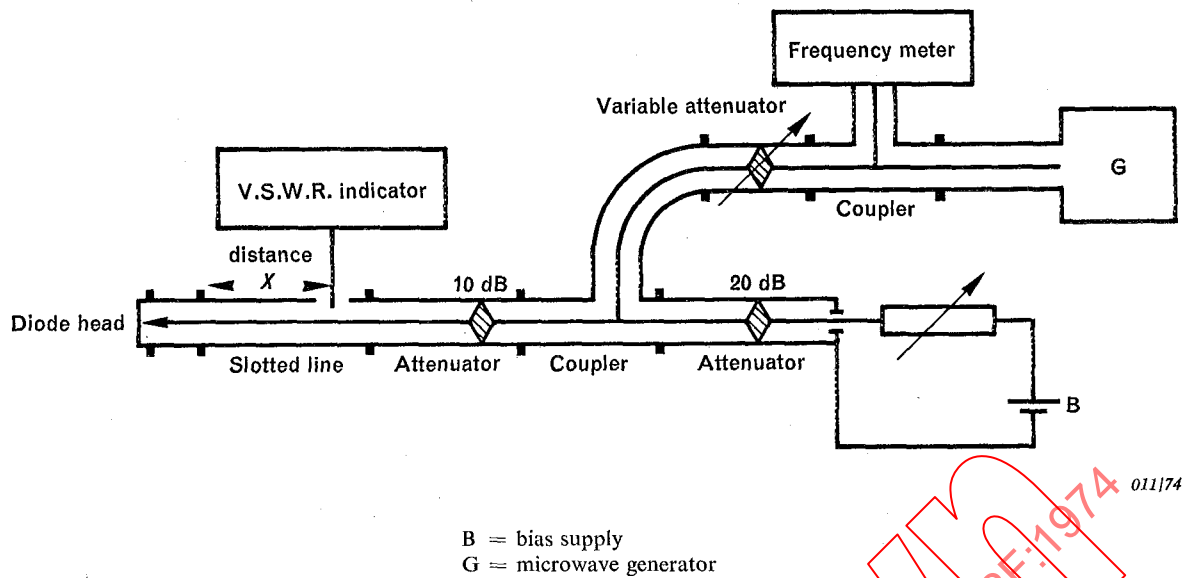
FIG. 9. — Equipment for measuring series inductance.
