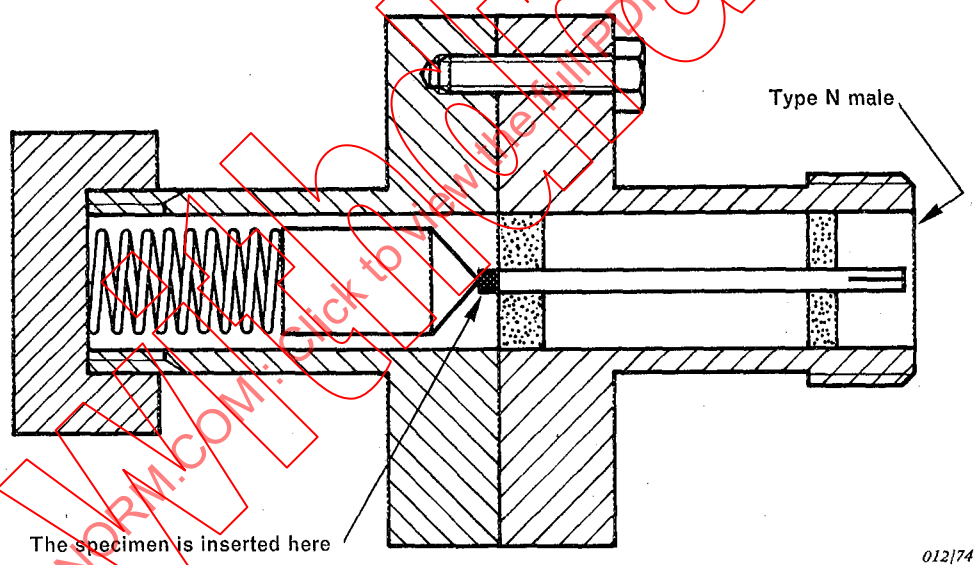
FIG. 10. — Diagram of measuring head.
