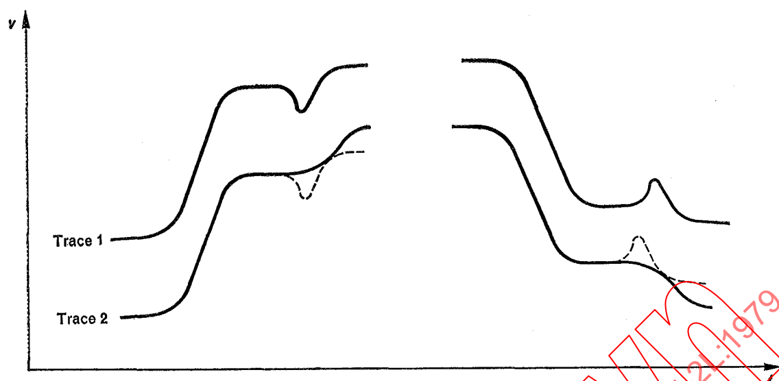
FIG. 8. — Non-coinciding traces due to disturbance of the balance by means of the circuit being measured (dotted lines show re-establishment of the balance by means of R_2 and C_2 ).
