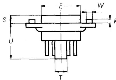
Type III: Montage sous chassis Under chassis mounting
