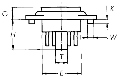
Type I: Montage sur chassis Over chassis mounting
