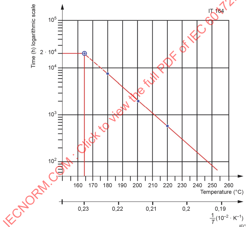
Figure 9 – Thermal endurance graph – Temperature index
