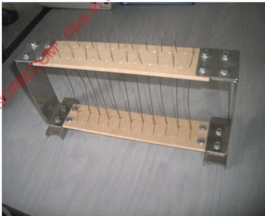
Figure 8 – Specimen holder
