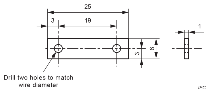
Figure 2 – Spacer
