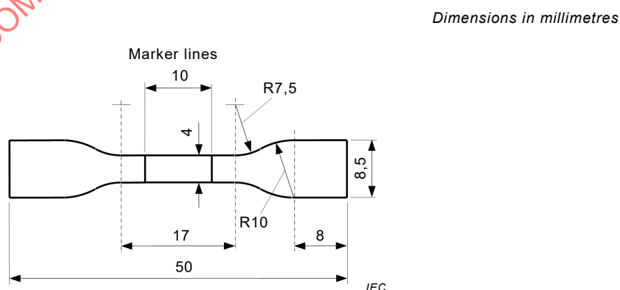
Figure 2 – Small dumb-bell test piece
