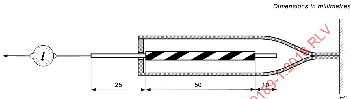
Figure 4 – Position of the sample in the test apparatus
