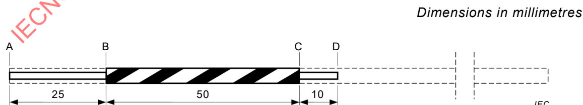
Figure 3 – Stripping properties of insulation
