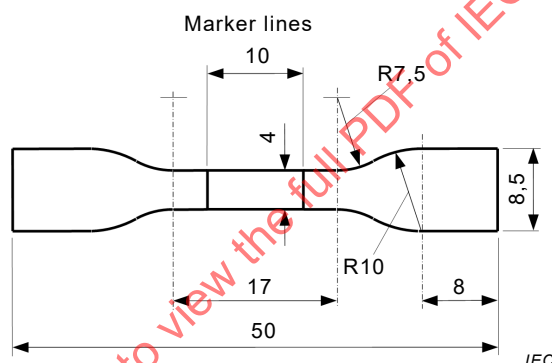
Figure 2 – Small dumb-bell test piece
