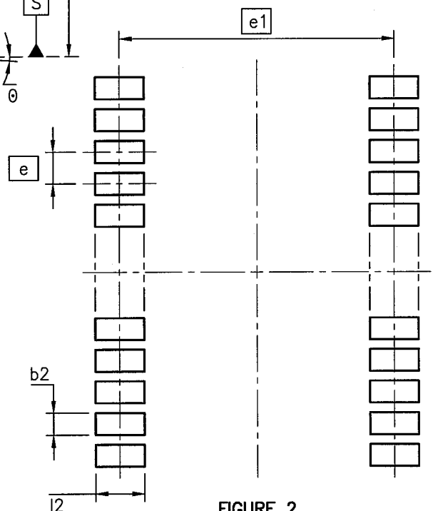
FIGURE 2 TERMINAL POSITION AREA (NOTE 4)
