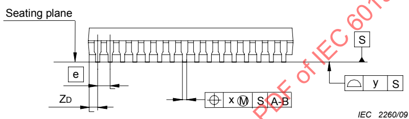
Figure 1c – Side view
