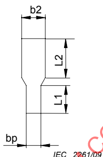
Figure A.9d - Lead shape
