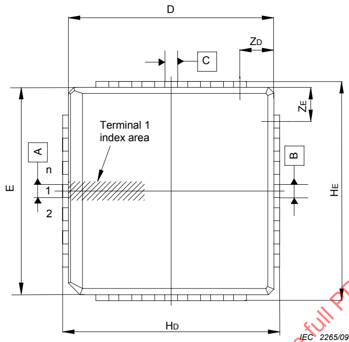
Figure A.11a – Top view
