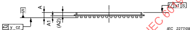
Figure A.15b – Side view
