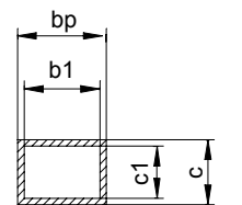
Figure A.9f - Lead section
