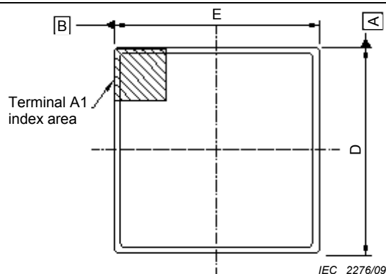
Figure A.15a – Top view
