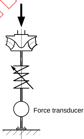
Figure 103 – Typical calibration arrangement for axial thrust measurement
