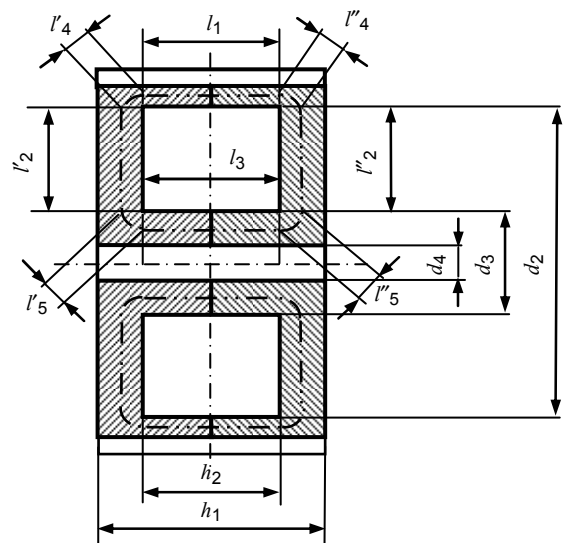
Section X-X
