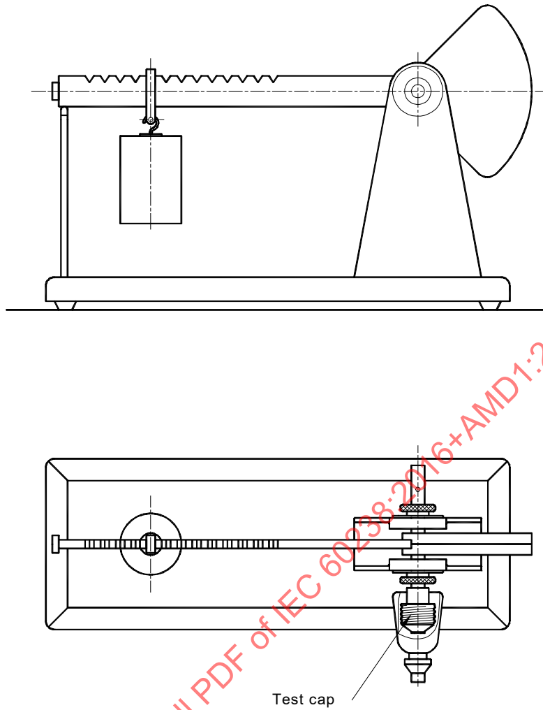
Figure 6 – Torque apparatus
