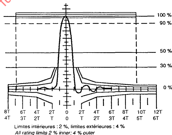
Figure 5e – Impulsion 2T/T Displayed 2T/T pulse signal
