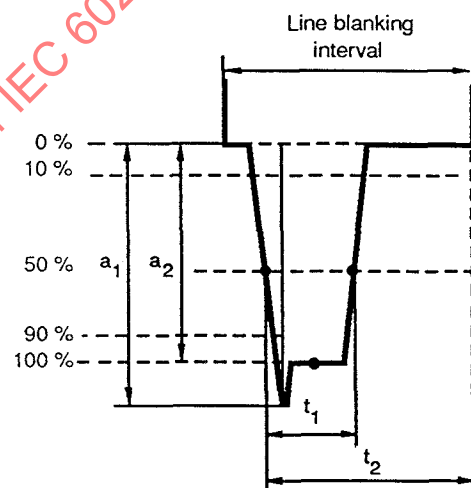
Figure 5k – Impulsion de synchronisation ligne Displayed line synchronizing pulse signal
