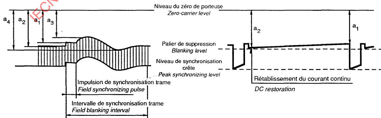
Figure 5l – Impulsion de synchronisation trame Displayed field-blanking interval signal
