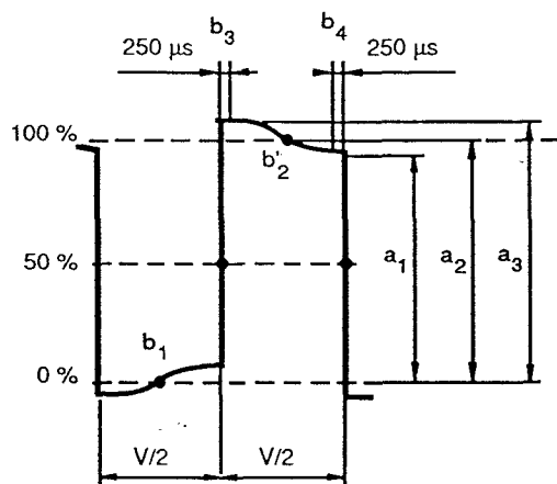
Figure 5h – Barre de trame Displayed field time bar signal
