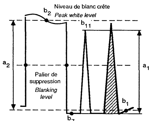
Figure 5b – Impulsion et signal de trame Displayed pulse and bar signal
