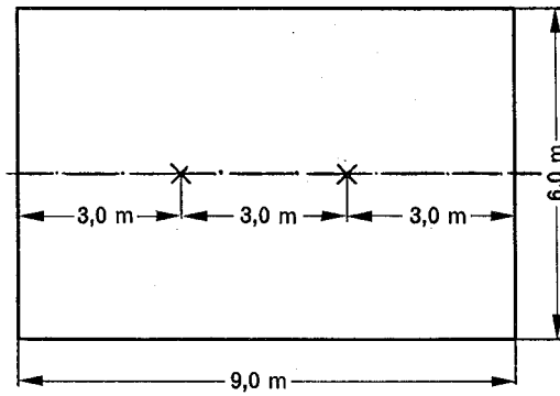
FIG. 1. — Grillage de sol. Wire mesh ground screen.
