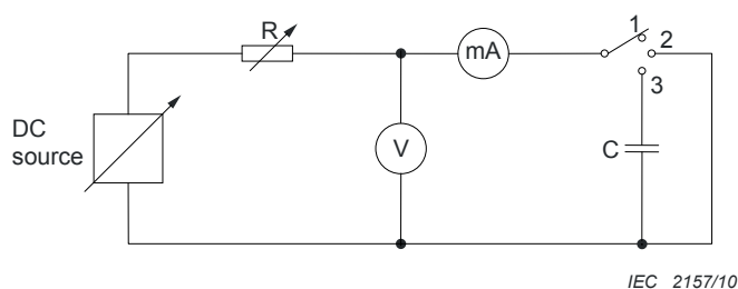
Figure 42 – Test apparatus for d.c. conditioning
