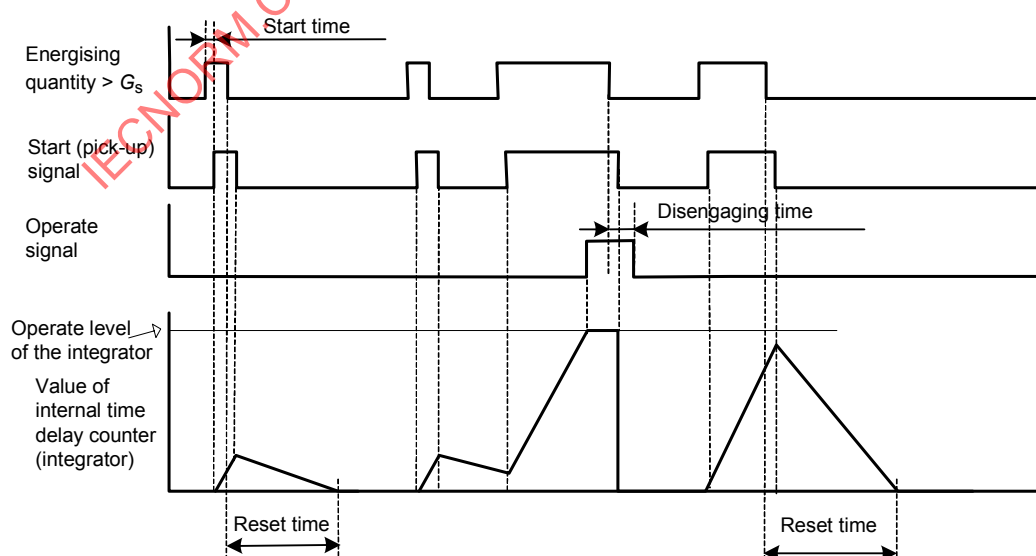
Figure 7 – Dependent time reset characteristic
