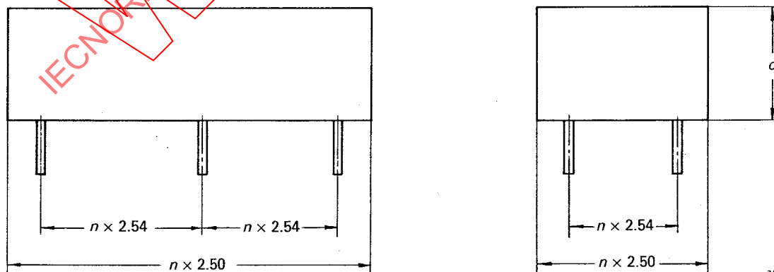
FIG. 5. — Example of relay for printed circuit board.
