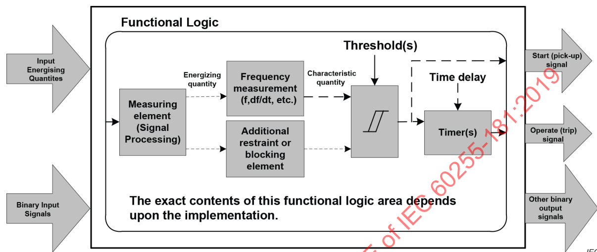
Figure 2 – Simplified protection function block diagram
