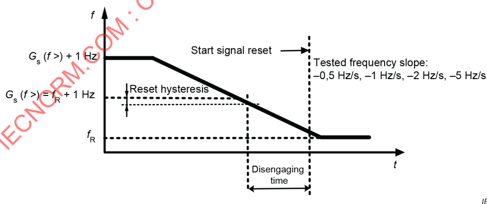
Figure 19 – Disengaging time measurement of overfrequency with constant slope frequency ramp
