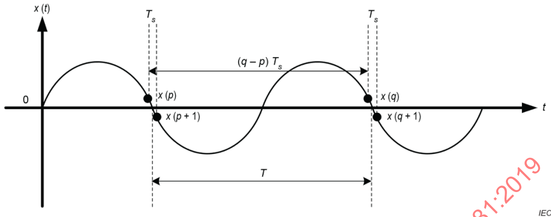
Figure C.1 – Zero-crossing algorithm
