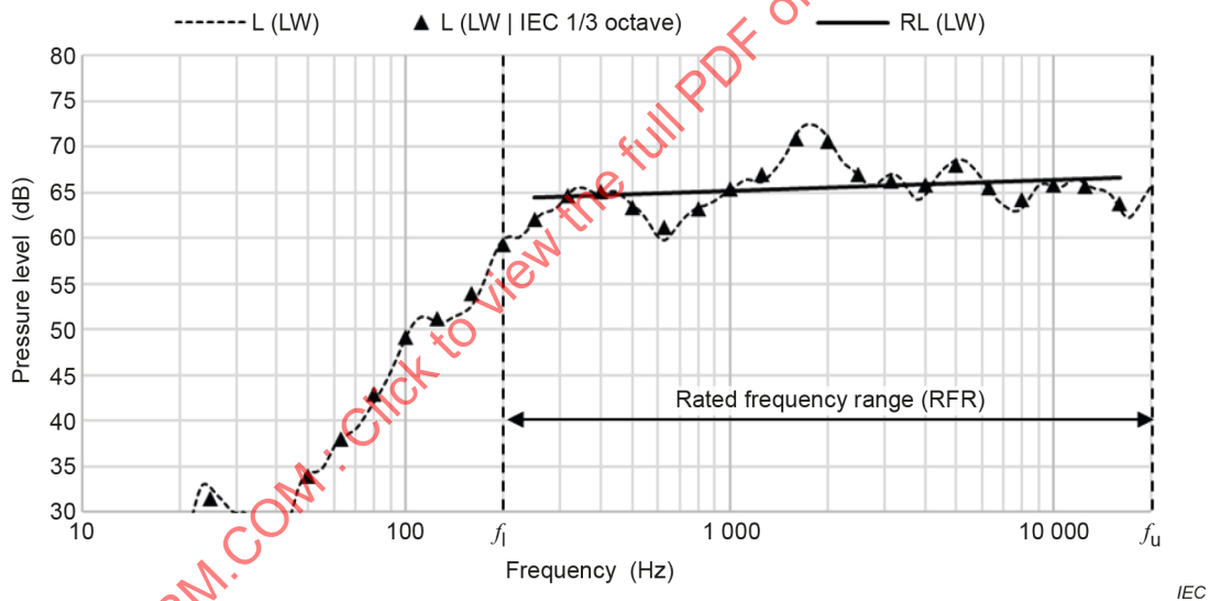
Figure 18 – Regression line deviation at rated frequency range
