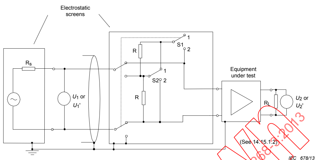
Figure 8 – Arrangement for measuring the balance of a balanced input
