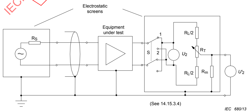
Figure 10 – Arrangement for measuring the voltage symmetry of a balanced output
