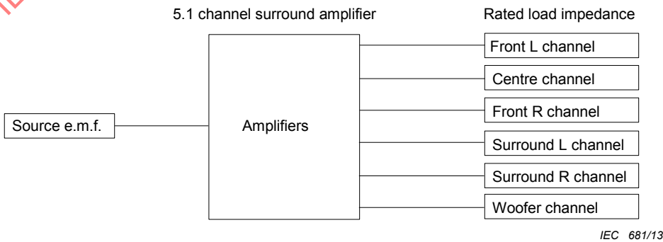
Figure B.1 – Block diagram for a 5.1 channel surround amplifier
