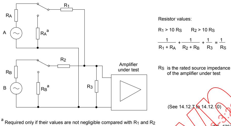
Figure 6 – Arrangement for combining two input signals
