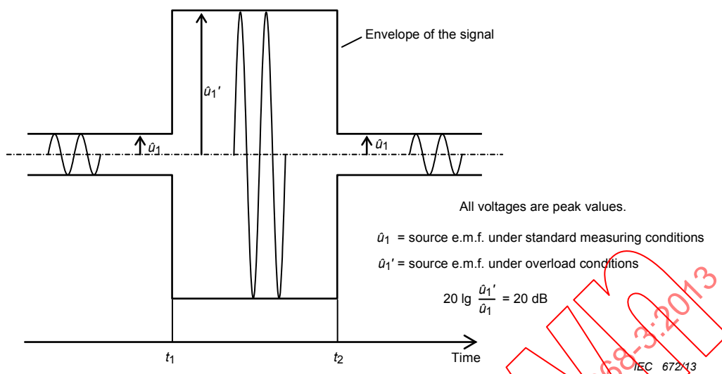
Figure 4a – Oscillogram of the source e.m.f. for measuring overload restoring time (see 14.6.5)
