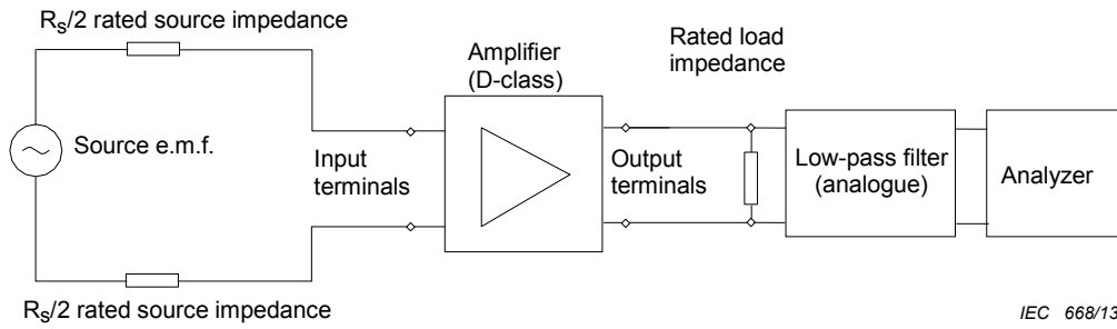
Figure 2a – Arrangements for the Class D amplifier – balanced input, floating (see 3.1.2)
