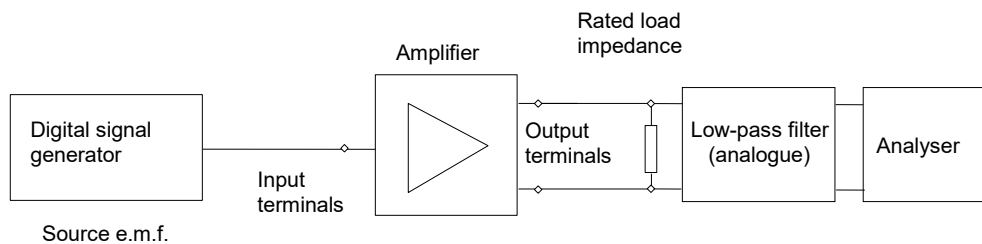
Figure 2 – Connection diagram of equipment for digital input
