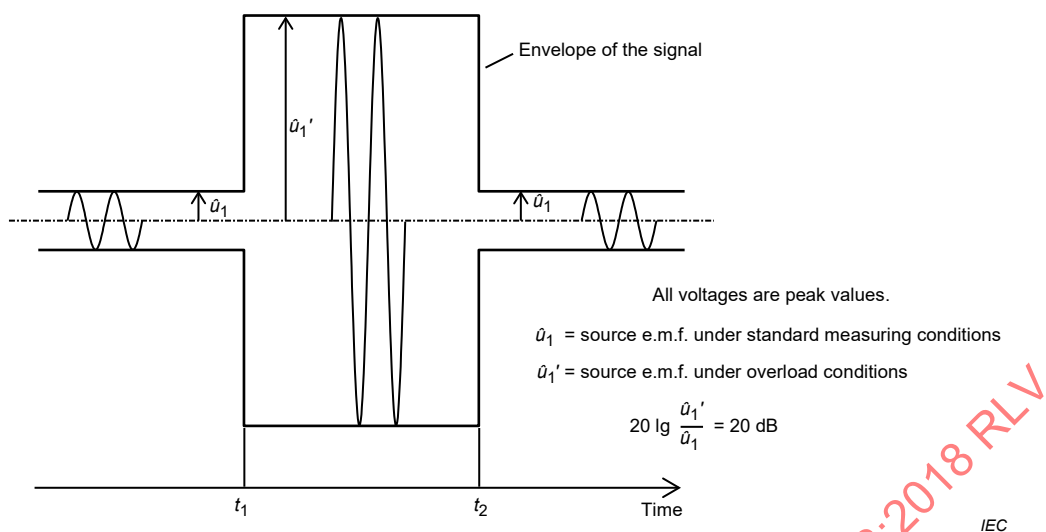
Figure 5a – Oscillogram of the source e.m.f. for measuring overload restoring time (see 15.6.6)
