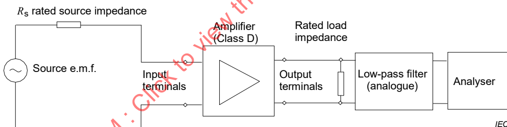
Figure 3b – Arrangements for the Class D amplifier – unbalanced input (see 4.1.2)
