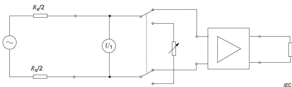
Figure 4a – Arrangements for measuring input impedance – balanced input, floating (see 15.5.2.2.2)
