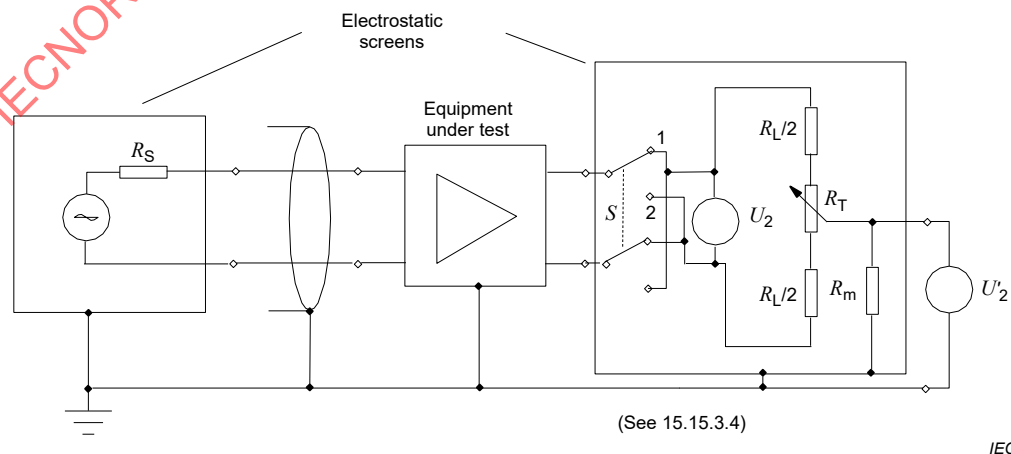
Figure 11 – Arrangement for measuring the voltage symmetry of a balanced output
