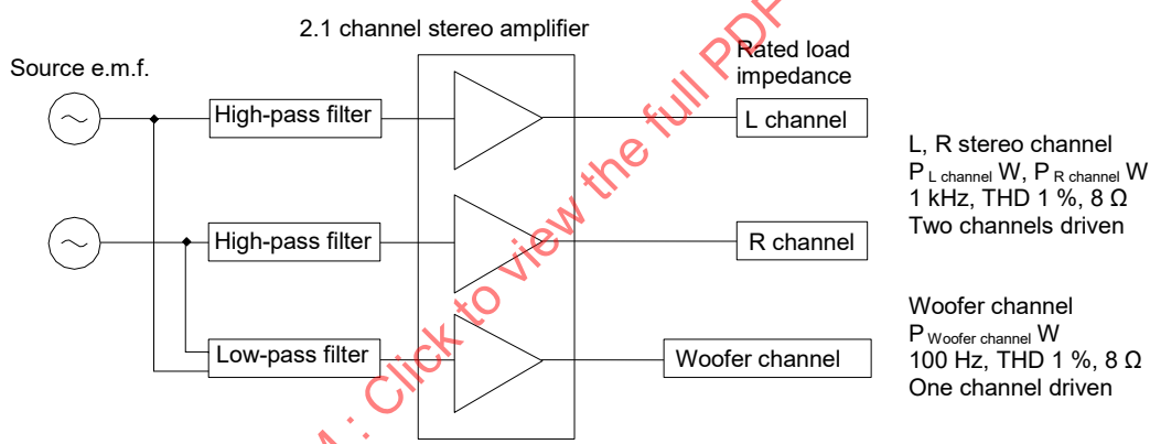
Figure 1b – Rated condition of 2.1 channel amplifiers (see 4.1.2)
