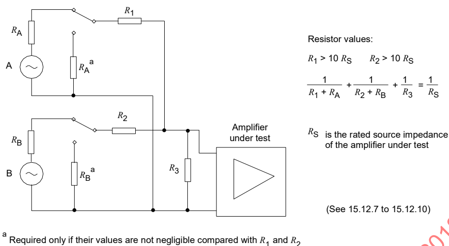
Figure 7 – Arrangement for combining two input signals
