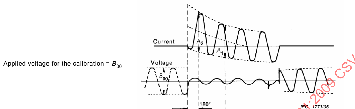
Figure 6a – Calibration of the circuit
