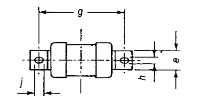
Size A fuse-link
