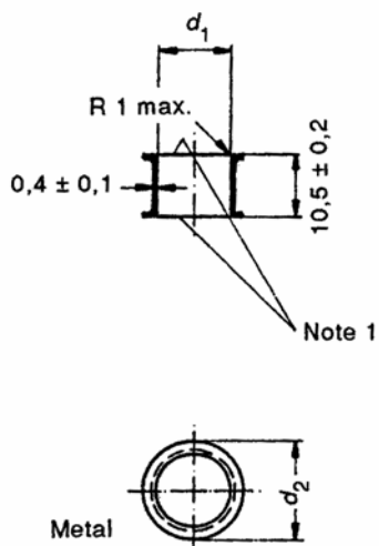
Gauge-piece D01/D02/D03
